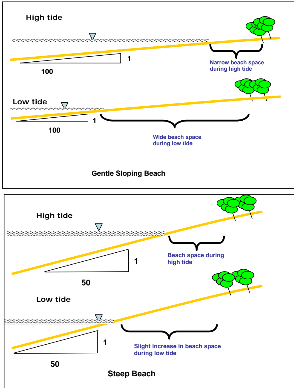
Figure 2: Changes in beach space for tidal range of 1 meter.
